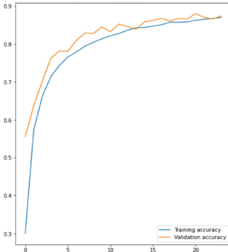
Fig 6: Validation accuracy
